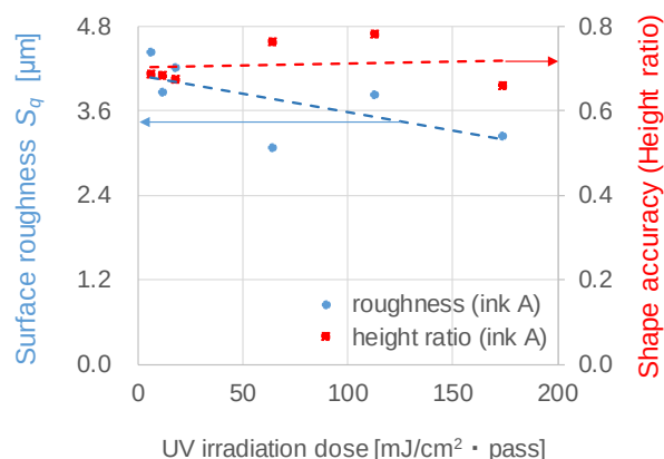
Fig. 5 Relationship of UV irradiation dose with surface roughness and shape accuracy in ink A (mono-functional monomer).
