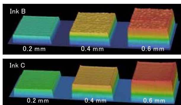
Fig. 10 3D imaging of stacking structures of ink B (above) and ink C (below) at heights of 0.2 mm, 0.4 mm, and 0.6 mm.
