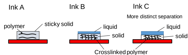
Fig. 11 Half-cured states.
