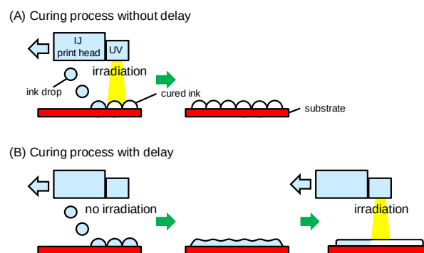
Fig. 14 Usual processes for (A) a rough surface and (B) a smooth surface.
