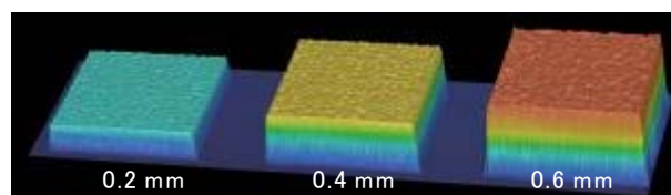
Fig. 3 3D imaging of stacking structures of ink A at heights of 0.2 mm, 0.4 mm, and 0.6 mm. *ten times magnification of height.
